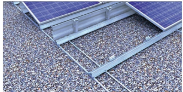
On gravel: south system I with gravel as ballast
