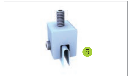
Clamp with VA saddle for copper standing seam roofs
